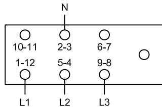
SERIES DELTA
