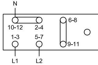
1 PHASE ZIG-ZAG
