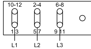
PARALLEL DELTA
