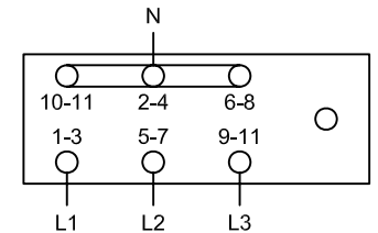
PARALLEL STAR
