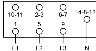
SERIES STAR
